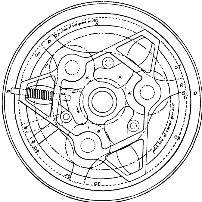
FIG. 356.—Front Elevation of the Duryea Change Speed Gear. The lettering here refers to the same parts as in the previous figure. N marks the position of the lever, M , when pins, P , are inserted in holes, Y , in D . M' marks the position of lever M when pins, P , are raised from holes in D . R and R' , arms of the spider, carrying the three idler pinions, A' , and sliding in a groove on H to the pins, T and T' .
